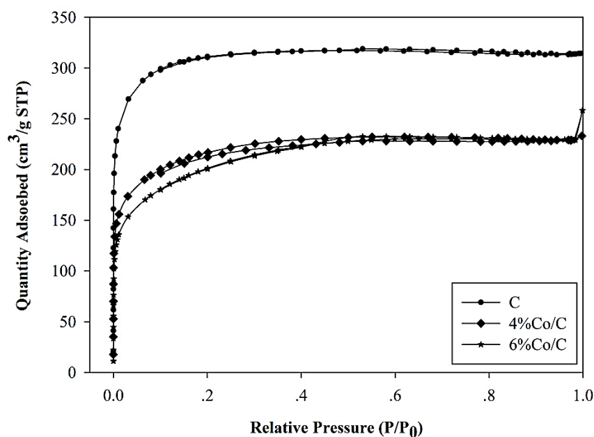
Fig. 1. Adsorption-desorption isotherm at -196°C of activated carbon-supported Co catalysts.
